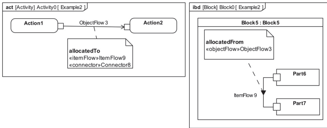
Figure 15-6: Example of flow allocation from ObjectFlow to ItemFlow
