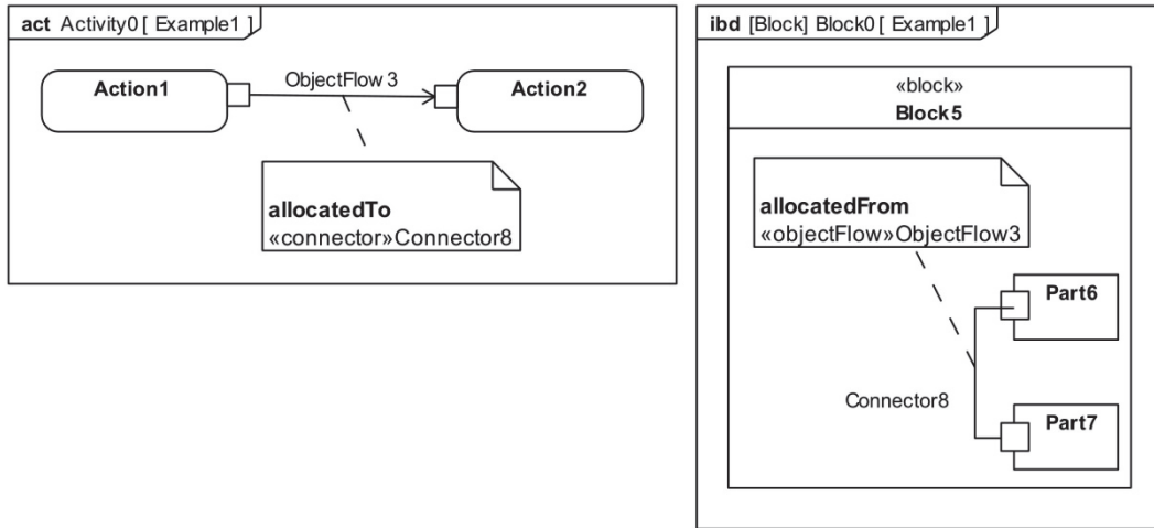
Figure 15-5: Example of flow allocation from ObjectFlow to Connector
