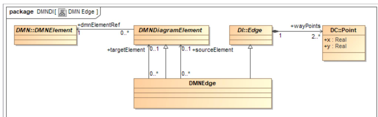
Figure 13.5: DMNEdge
