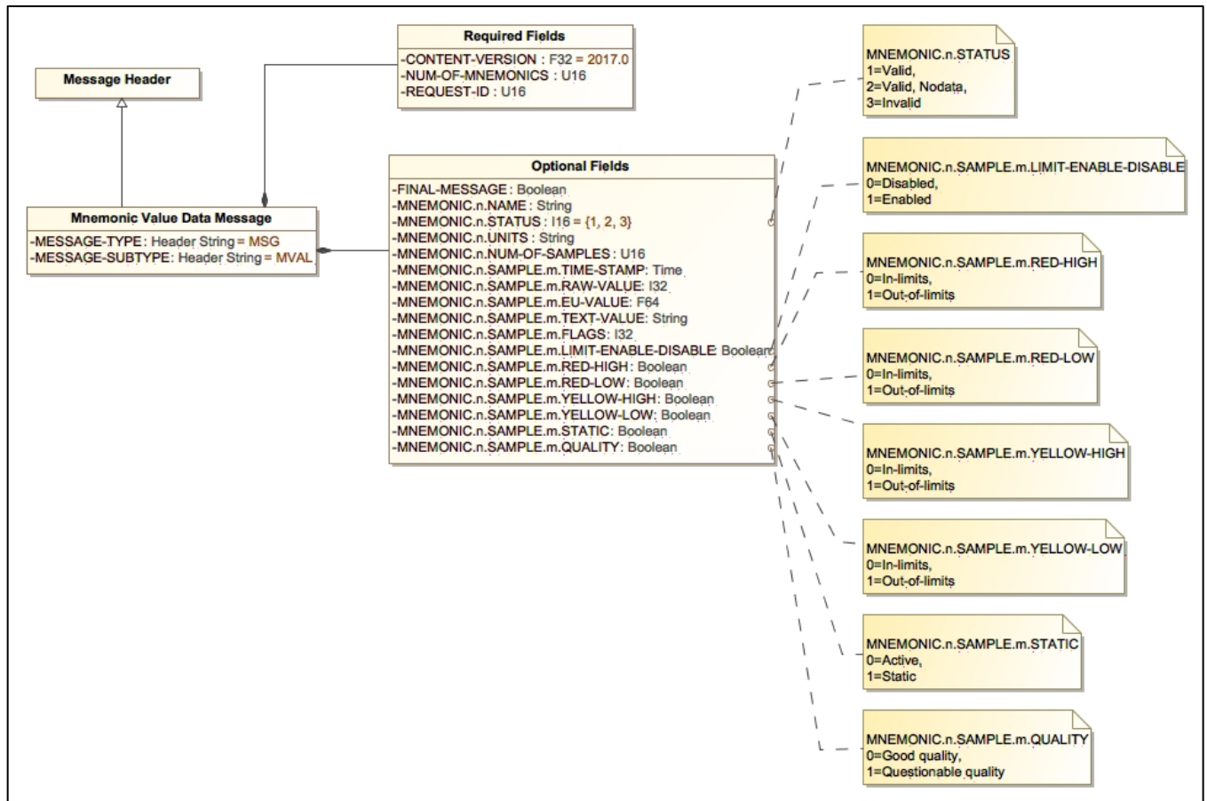
Figure 8-22. Mnemonic Value Data Message Diagram
