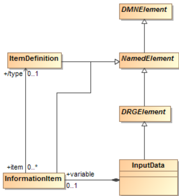
Figure 236-42: InputData class diagram
