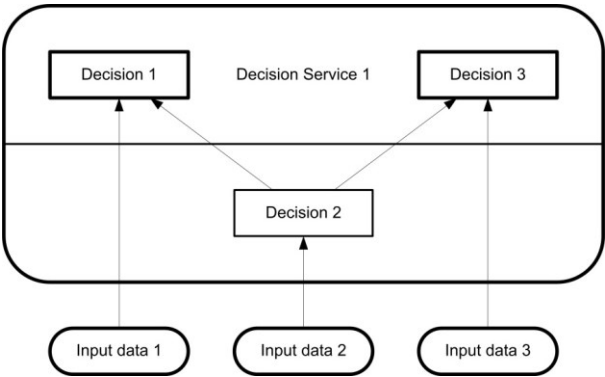
Figure 176-6: Decision Service notation
