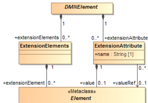
Figure 256-14: Extensibility class diagram
