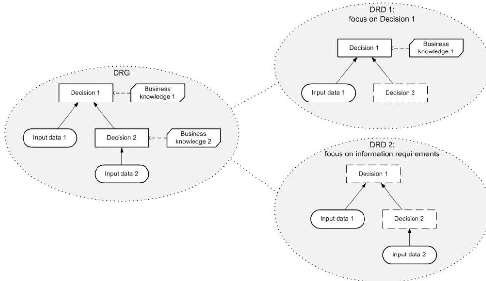
Figure 166.5: DRDs as partial views of a DRG
