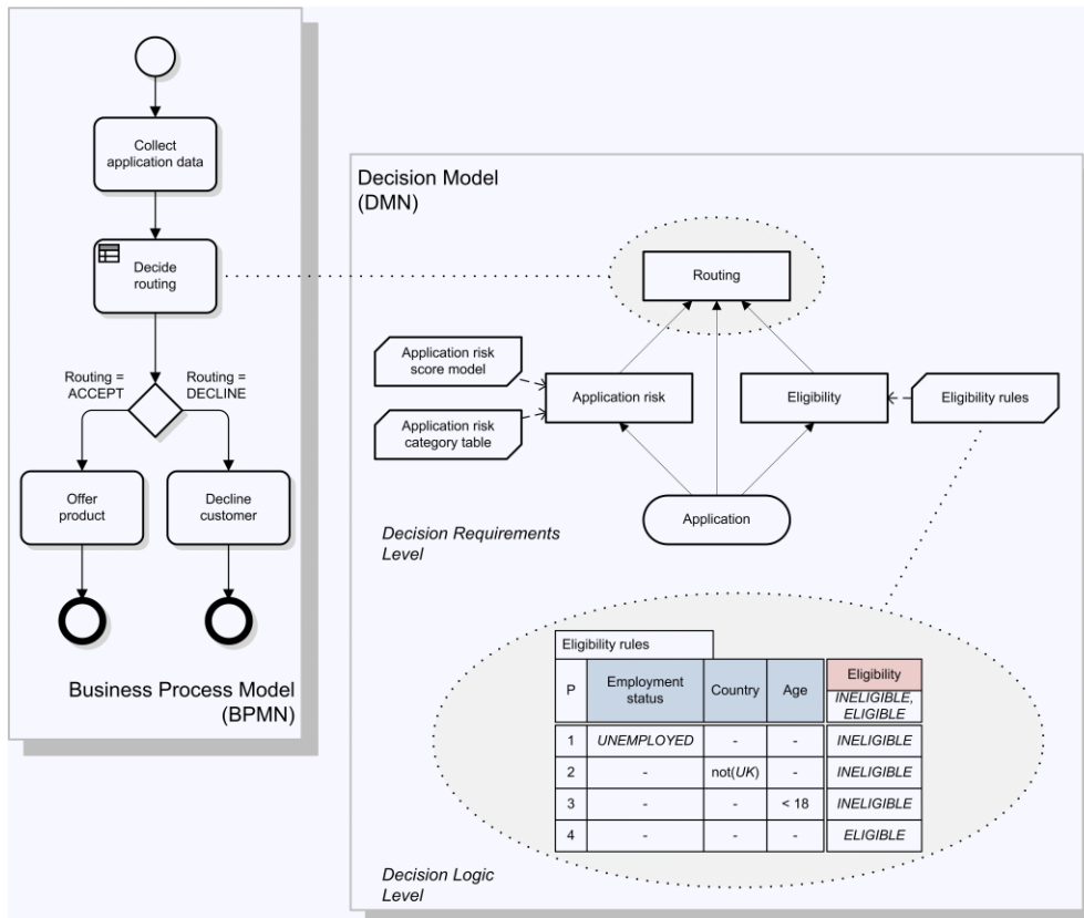
Figure 15.1 - Aspects of Modeling
