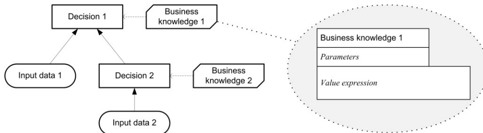
Figure 85.8: Business knowledge model and corresponding value expression
