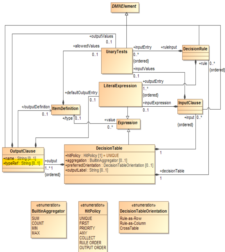
Figure 518-20: DecisionTable class diagram
