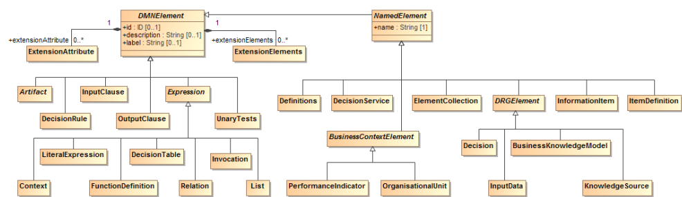
Figure 186-7: DMNElement Class Diagram
