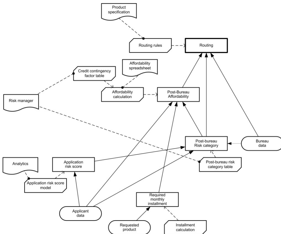
Figure 714.4: DRD for Decide routing decision point
