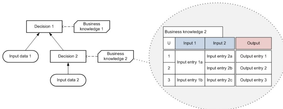
Figure 95.9: Business knowledge model and corresponding decision table
