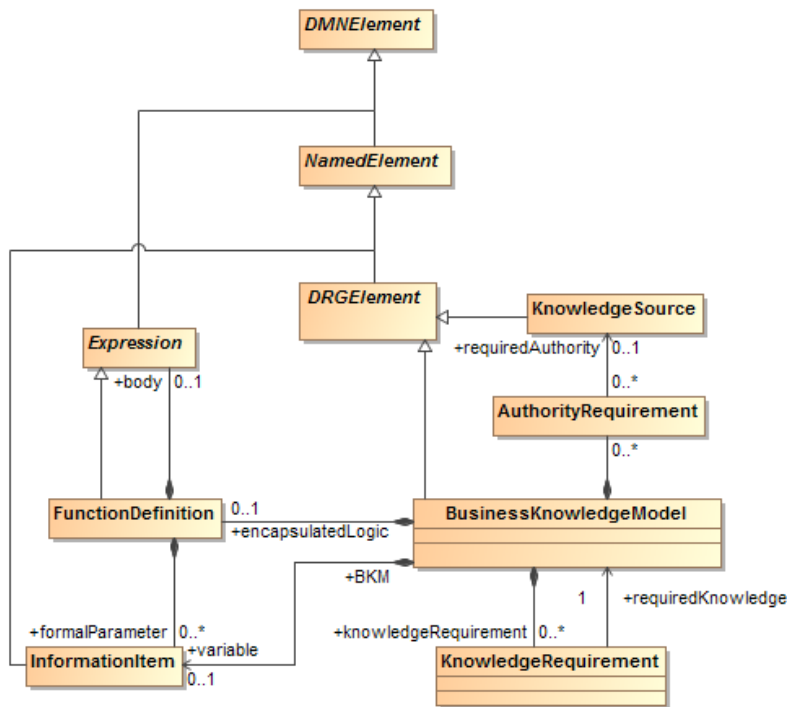
Figure 226-44: BusinessKnowledgeModel class diagram
