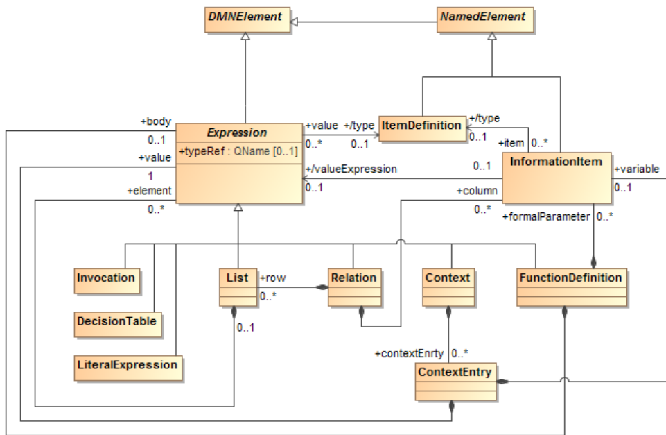
Figure 10.5 - Expression class diagram
