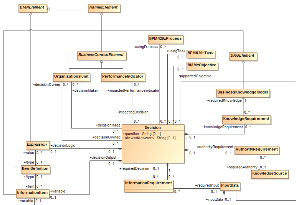
Figure 206.9: Decision Class Diagram
