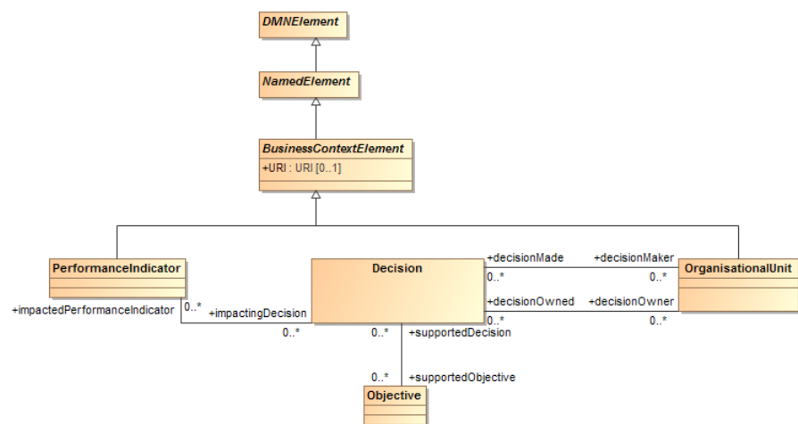
Figure 216.10: BusinessContextElement class diagram
