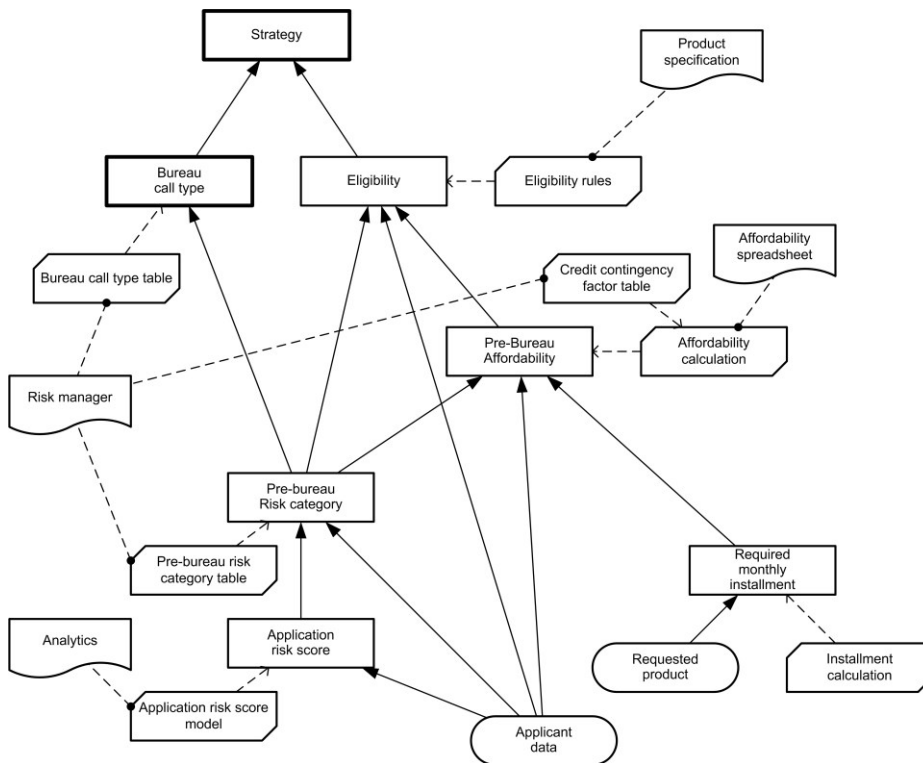
Figure 6911.3: DRD for Decide bureau strategy decision point
