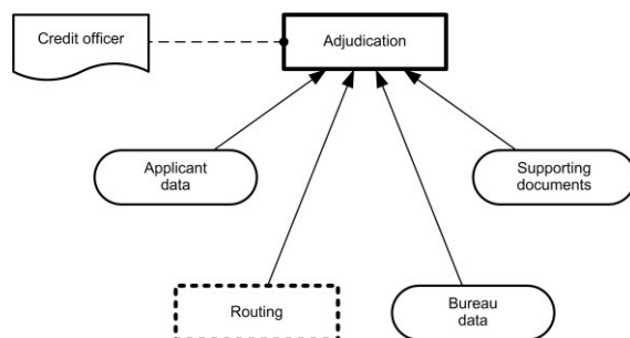
Figure 714.5: DRD for Review application decision point
