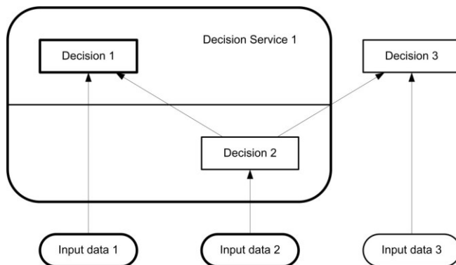
Figure 105-10: A decision service
