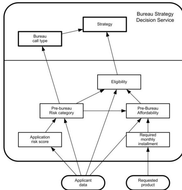
Figure 7244.6: Bureau Strategy Decision Service
