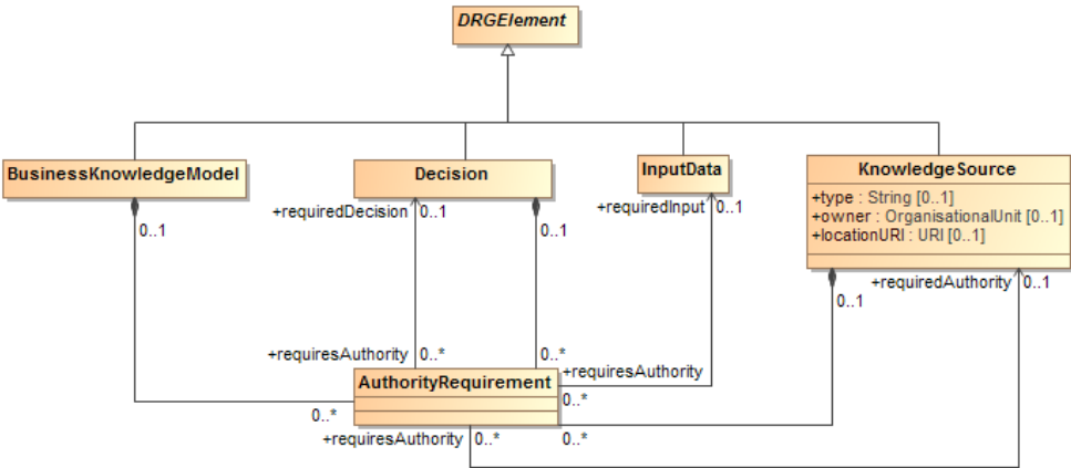
Figure 246-13: KnowledgeSource class diagram
