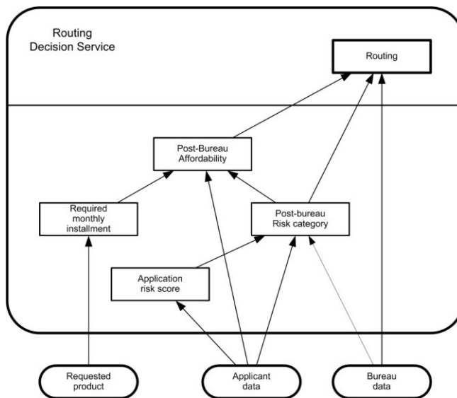
Figure 7344.7: Routing Decision Service
