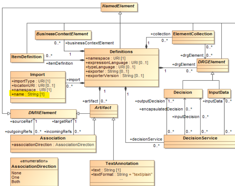
Figure 196-8: Definitions Class Diagram
