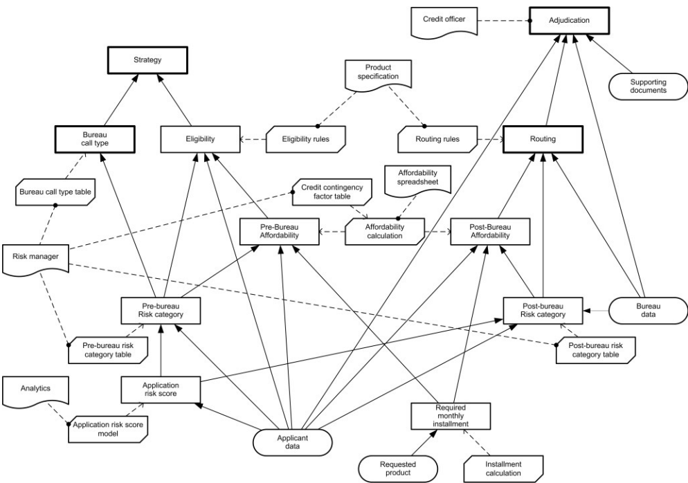
Figure 6841-2: DRD of all automated decision-making
