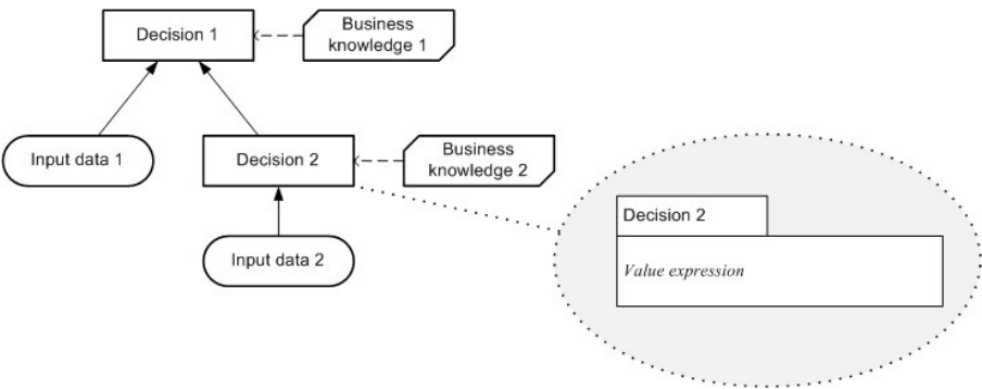
Figure 75-7: Decision and corresponding value expression
