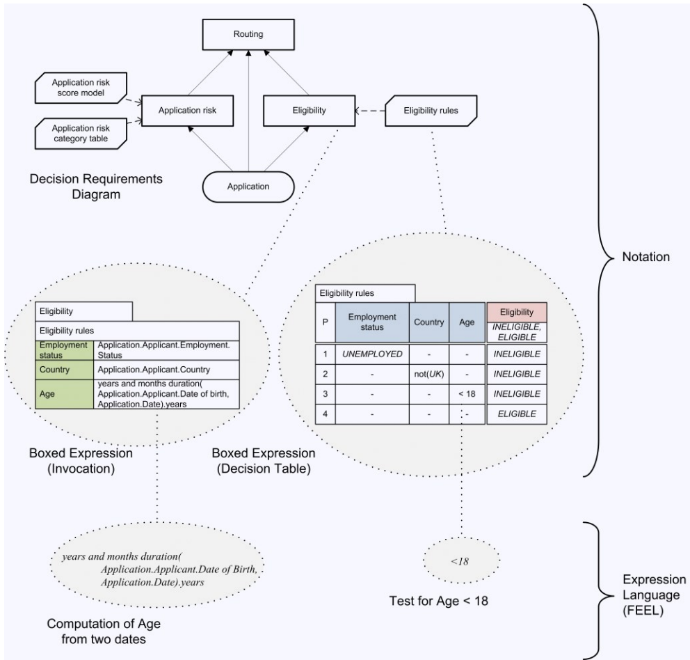
Figure 25.2: DMN Constructs
