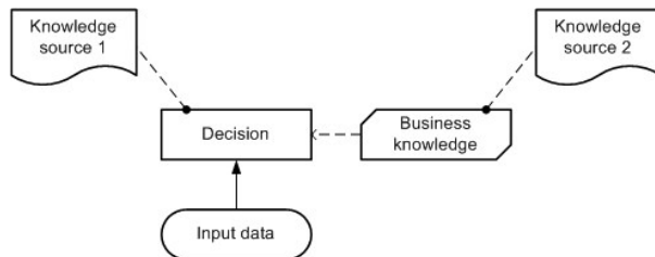
Figure 45.4: Knowledge sources
