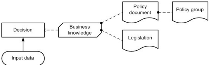
Figure 146-3: Knowledge Sources representing authorities
