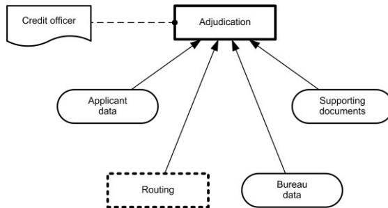
Figure 7144.5: DRD for Review application decision point
