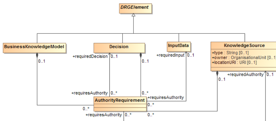
Figure 246-13: KnowledgeSource class diagram
