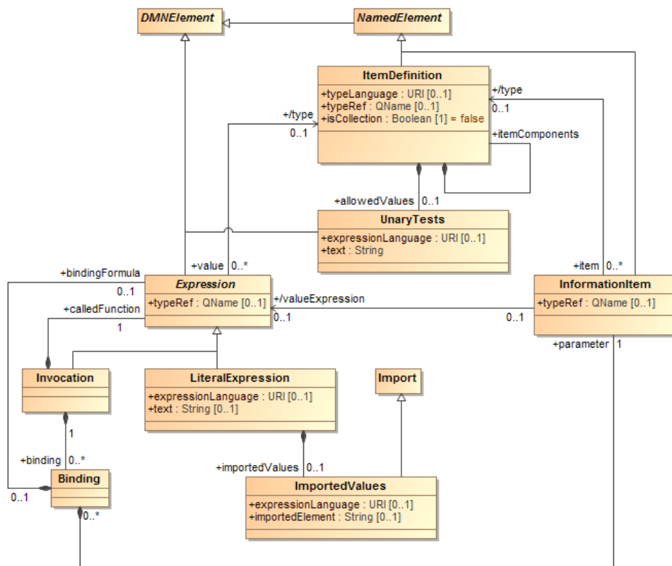
Figure 317-6: Expression class diagram
