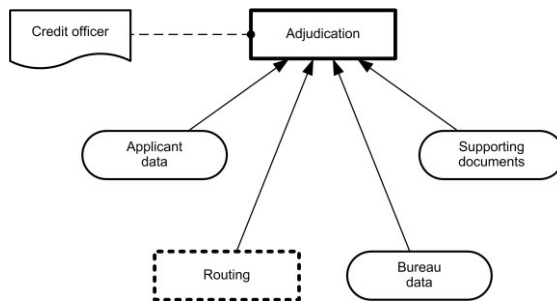
Figure 7144.5: DRD for Review application decision point
