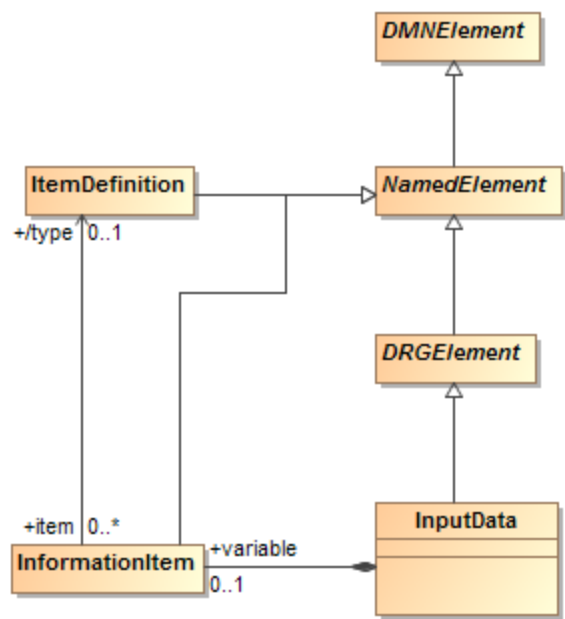
Figure 236-12: InputData class diagram
