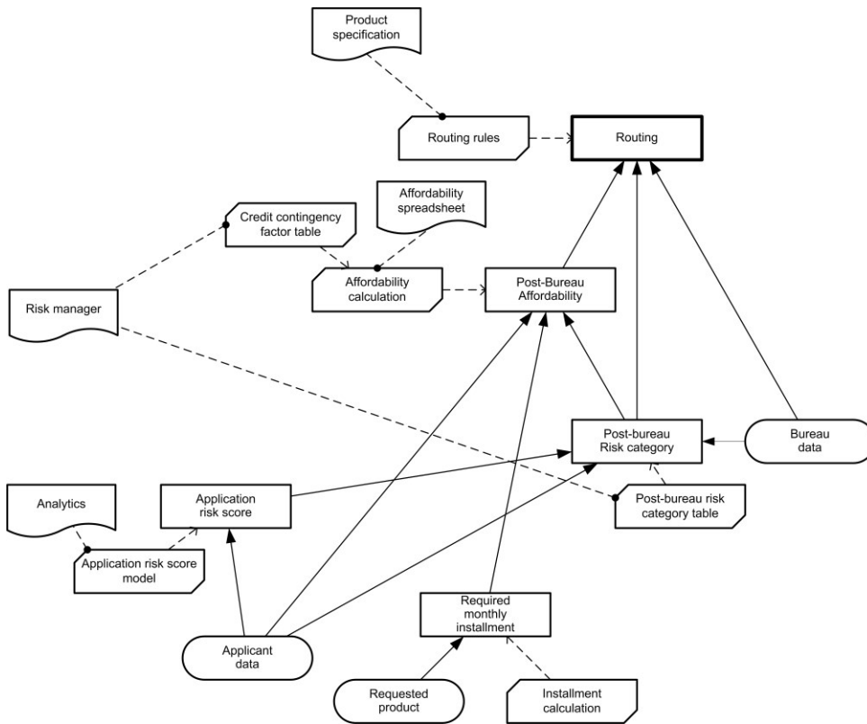
Figure 7044.4: DRD for Decide routing decision point
