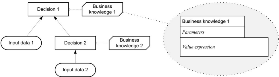
Figure 95-8: Business knowledge model and corresponding value expression
