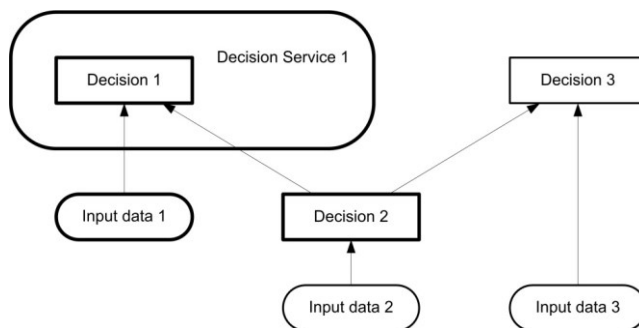
Figure 115-44: A decision service taking a decision as input
