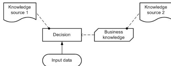
Figure 45-4: Knowledge sources
