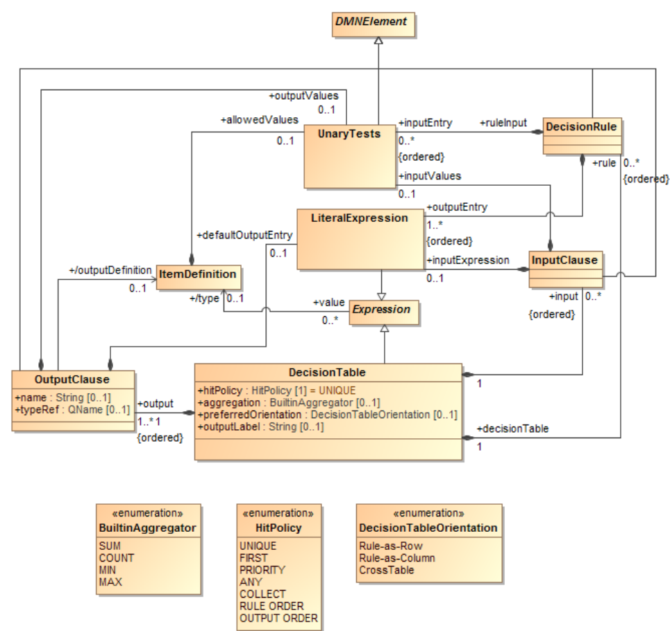
Figure 518-20: DecisionTable class diagram
