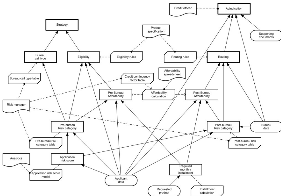
Figure 6844.2: DRD of all automated decision-making
