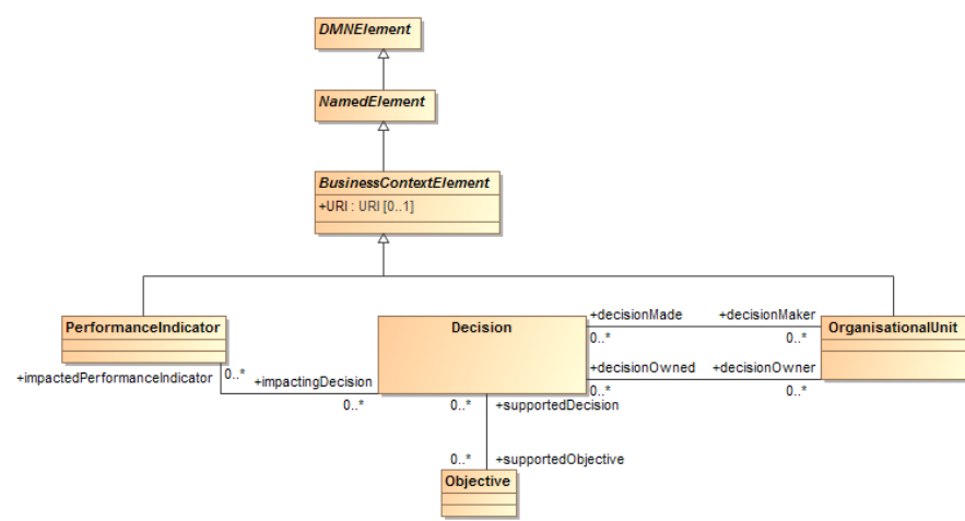
Figure 216-10: BusinessContextElement class diagram
