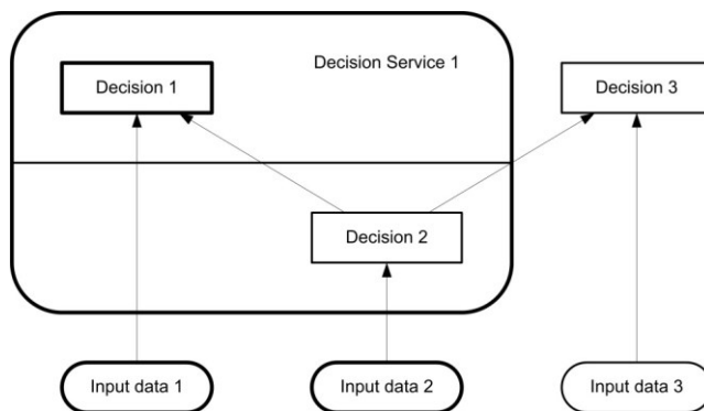
Figure 105-40: A decision service
