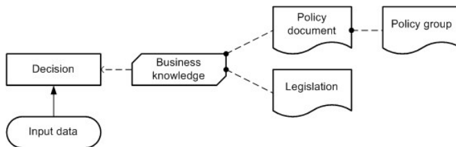
Figure 146-3: Knowledge Sources representing authorities
