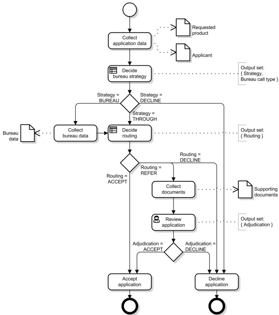
Figure 6744-1: Example business process
