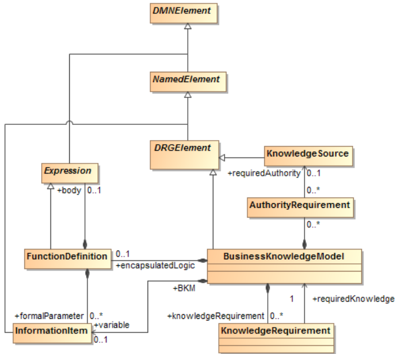
Figure 226-11: BusinessKnowledgeModel class diagram
