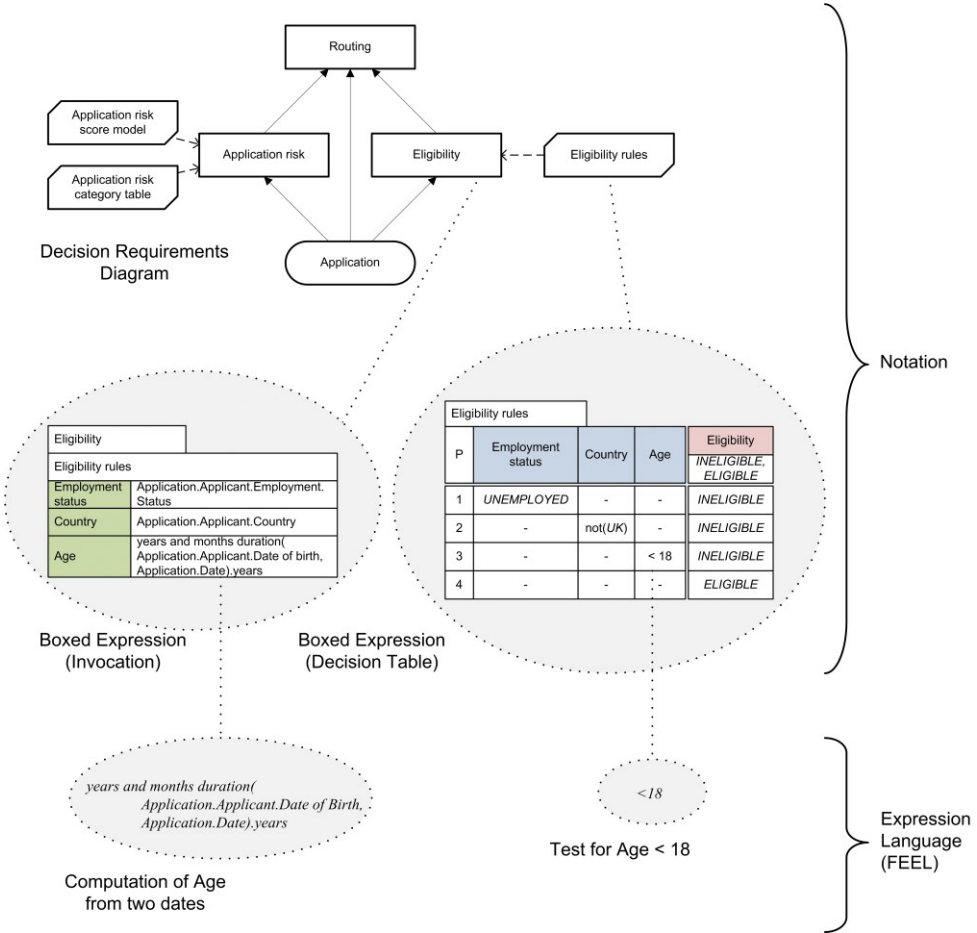
Figure 2.5-2: DMN Constructs
