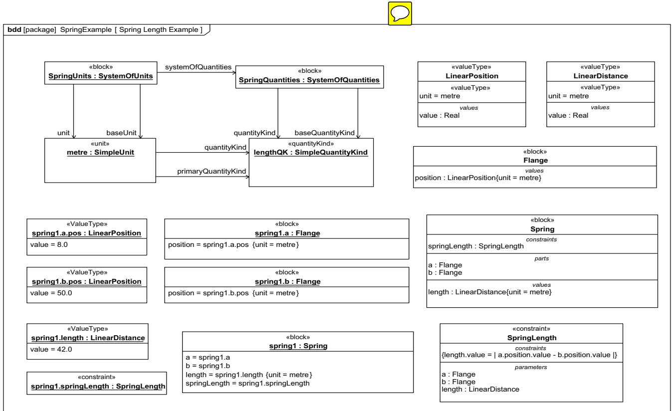
Figure E.9 - Spring Length Example
